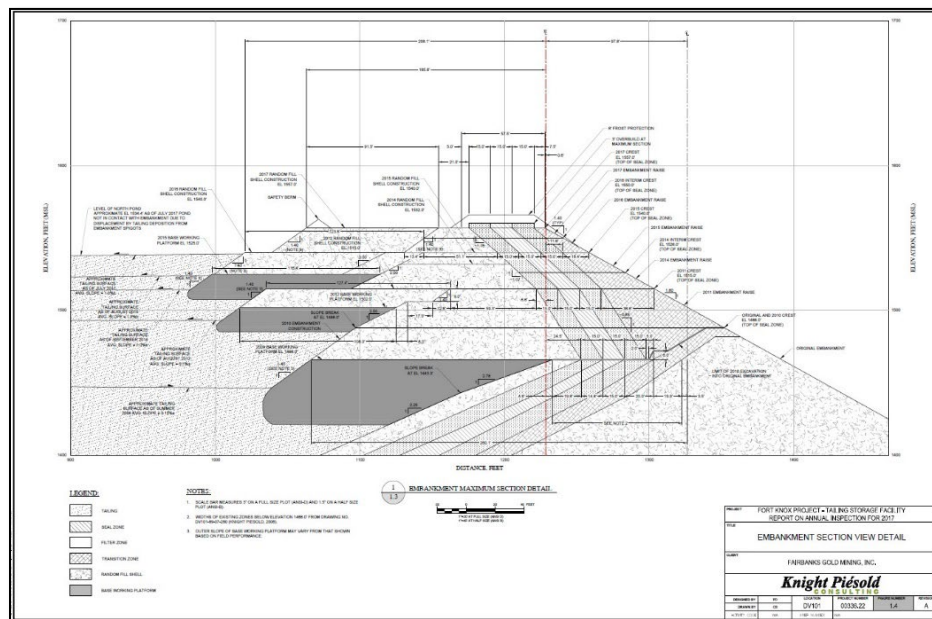
Figure 11: TSF Modified Centerline Design
