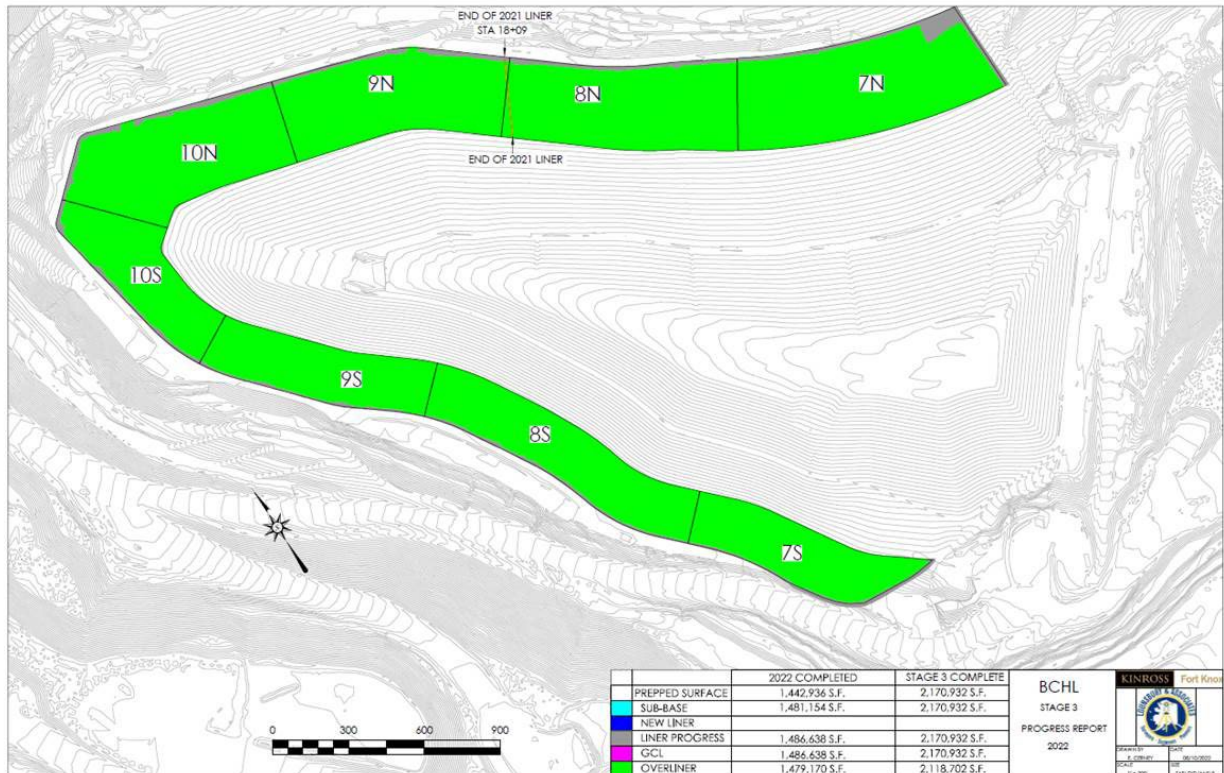
Figure 8: Barnes Creek Heap Leach Stage 3 Progress in 2022
