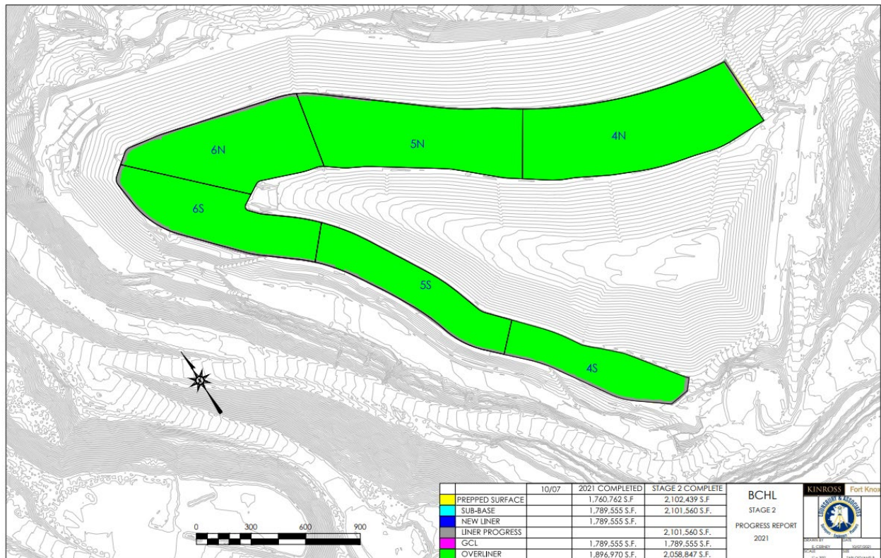
Figure 6: Barnes Creek Heap Leach Stage 2 Progress in 2021
