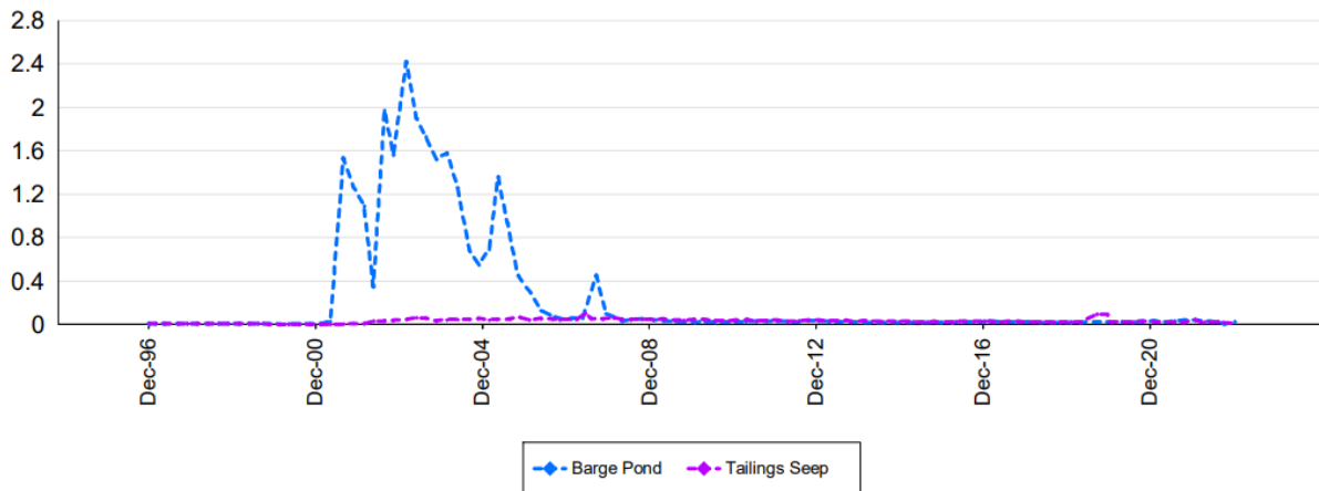
Figure 14: Average Quarterly Antimony Concentrations in Seepage Reclaim & Decant
