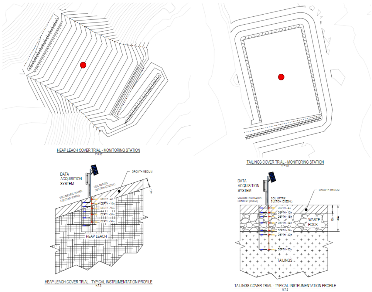
Figure 18: Cover Trial Instrumentation Details
