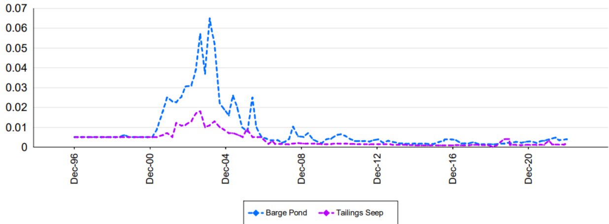
Figure 17: Average Quarterly Selenium Concentrations in Seepage Reclaim & Decant
