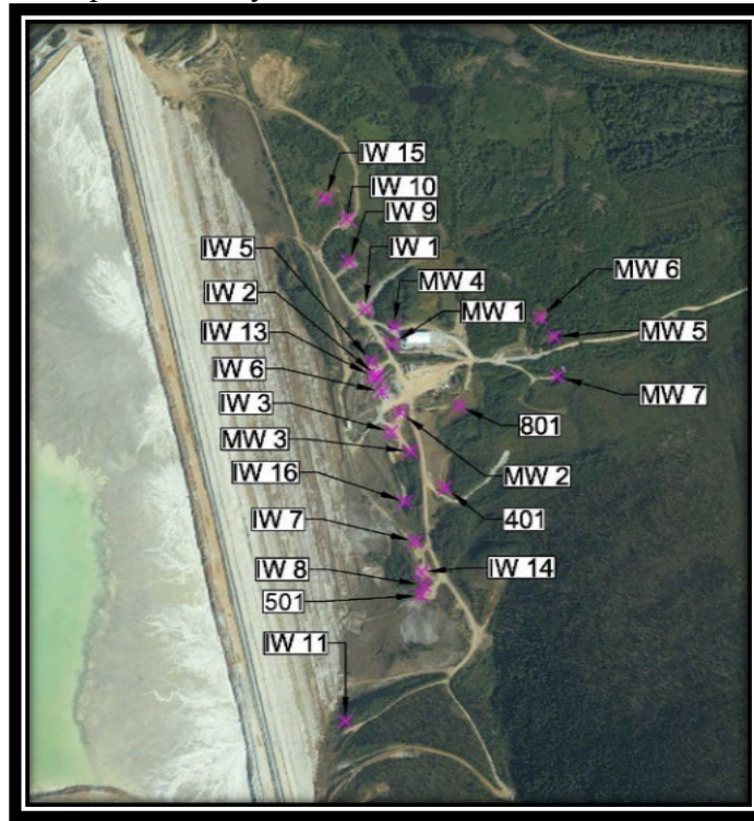
Figure 8: Operating Interceptor Well System
