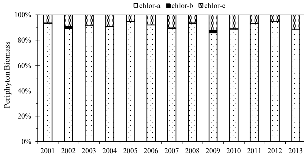
Figure 17.—Greens Creek Site 54 proportions of mean chlorophylls a , b , and c densities, 2001–2013.
