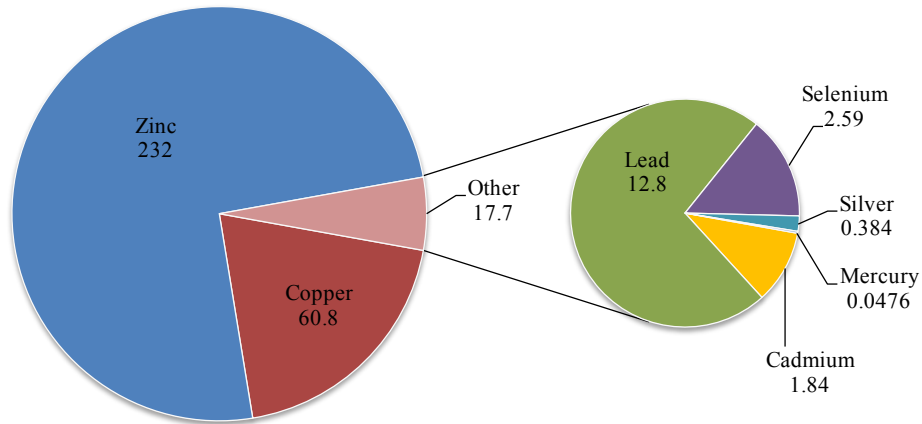
Figure 15.–Greens Creek Site 48 sediment metals and Se concentrations (mg/kg), 2013.
