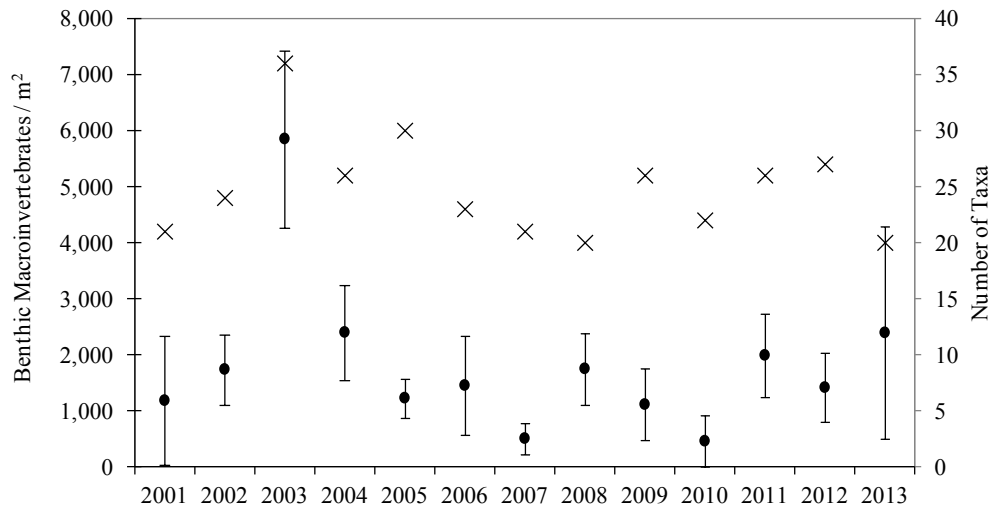
Figure 27.—Tributary Creek Site 9 mean benthic macroinvertebrate density \pm one standard deviation, and taxa richness (×), 2001–2013.
