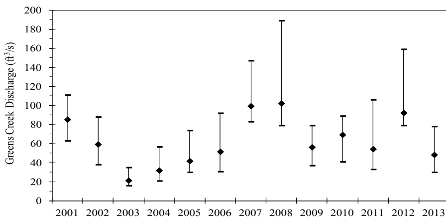
Figure 7.—Greens Creek (USGS Gage 15101490) range of mean daily discharges (ft 3 /s), and the median value (♦), three weeks prior to sampling, 2001–2013. Source: USGS Gage 15101490 (USGS 2014).
