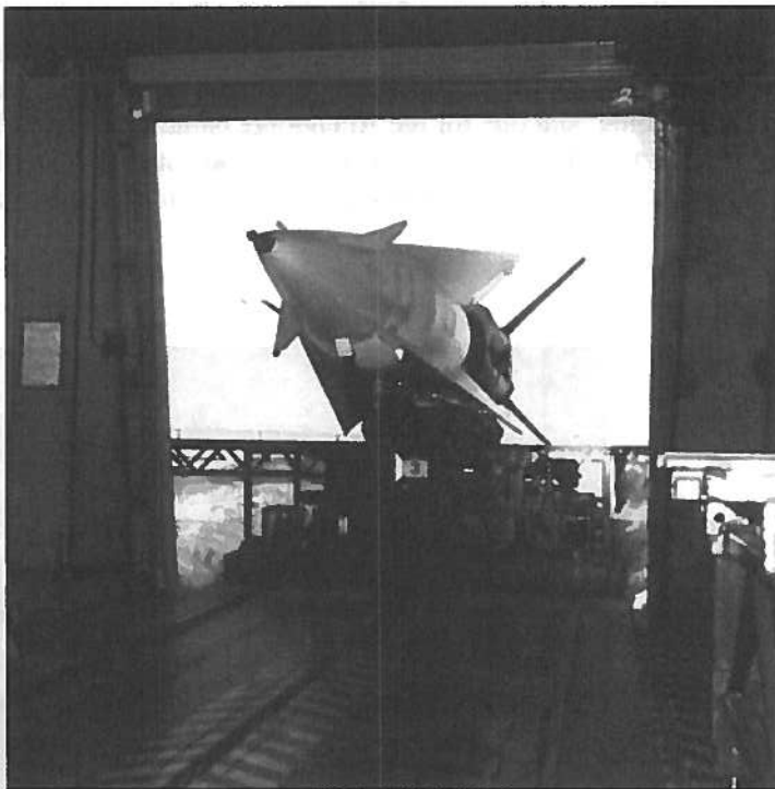
Figure 3: Nike Hercules Rollout to Firing, February 1968, Site Summit, Anchorage. U.S. Army Photo.
